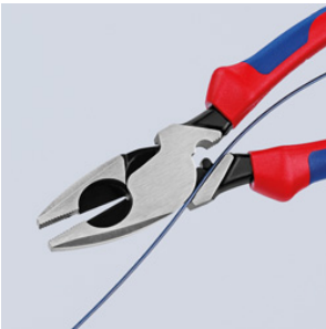
09 11/12 240: fish tape puller in the joint gap
