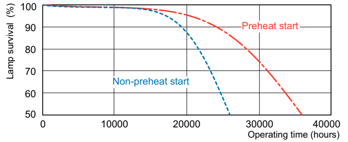
MASTER TL5 HO EcoPlus Life Expectancy 12 h cycle
