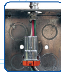
Pull conduit thru knockout, insert wires in fitting
