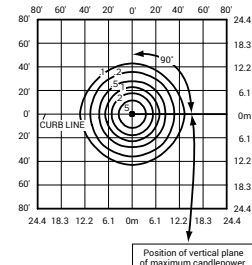
CPY250-A-**-D-A-UL Mounting Height: 15' (4.6m) Initial Delivered Lumens: 8,000 Initial FC at grade
