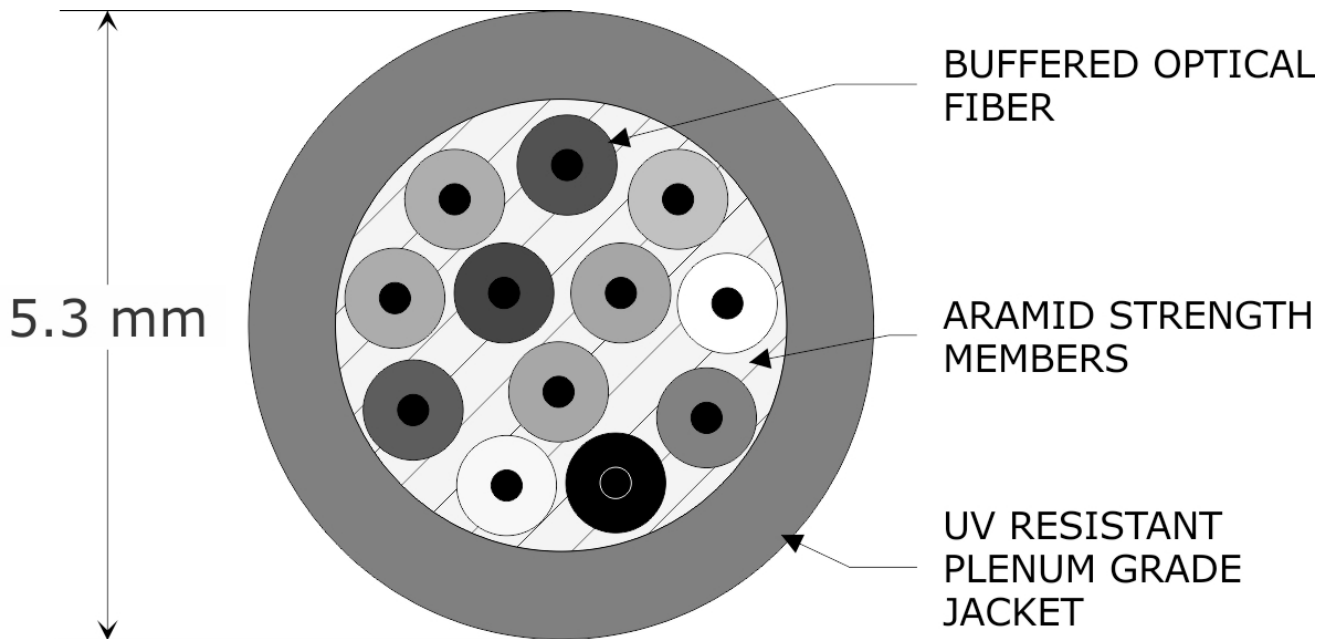
Cross-section Diagram - PDP012-I/O
