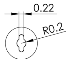
DETAIL A SCALE 2 : 5
