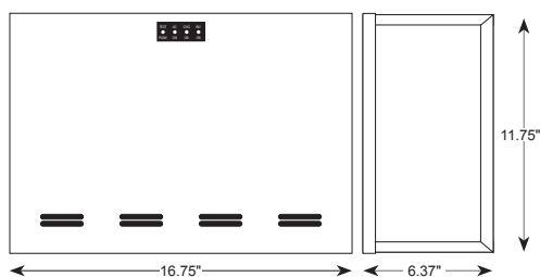
LG250S AND LG250SI WALL MOUNT SURFACE MODELS
