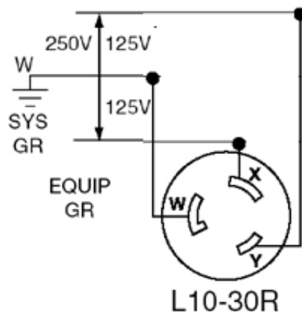
Wiring Diagram
