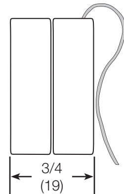
Transmitter (Side)
