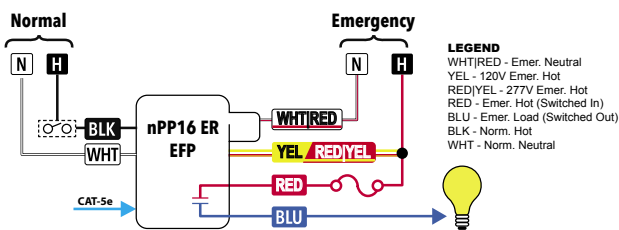
Diagram for non-dimming units
