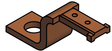
VIEW9 SCALE 2 : 1
