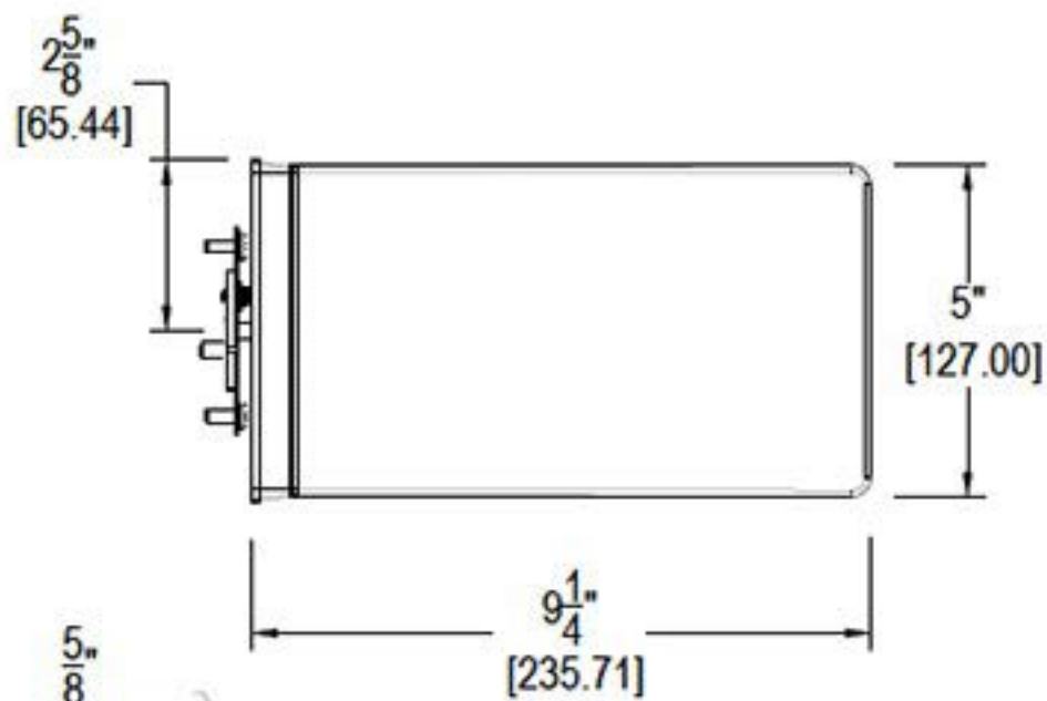
Surface Mount Configuration
