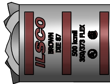
DETAIL A TOP AND BOTTOM INK MARKINGS ARE IDENTICAL INK COLOR:BROWN PER SPEC #: F921
