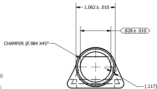
DETAIL A TOP AND BOTTOM INK MARKINGS ARE IDENTICAL INK COLOR:BROWN PER SPEC #: F921
