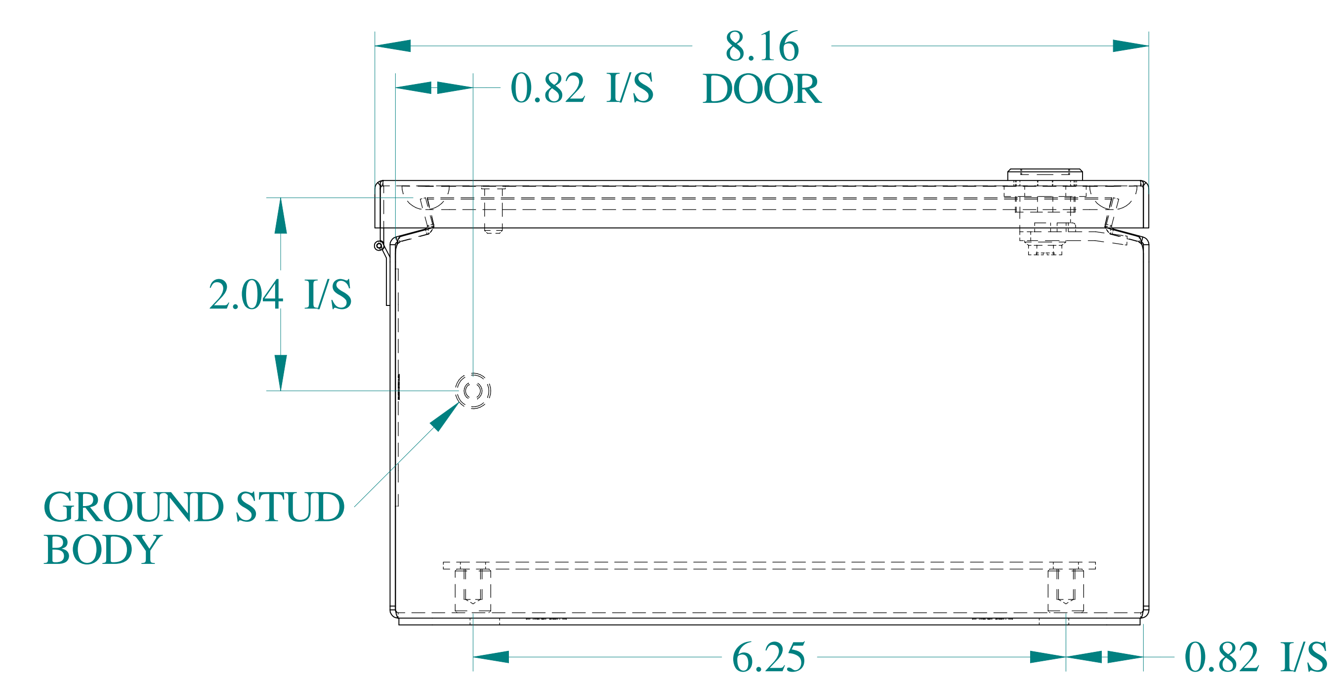
BOTTOM VIEW
