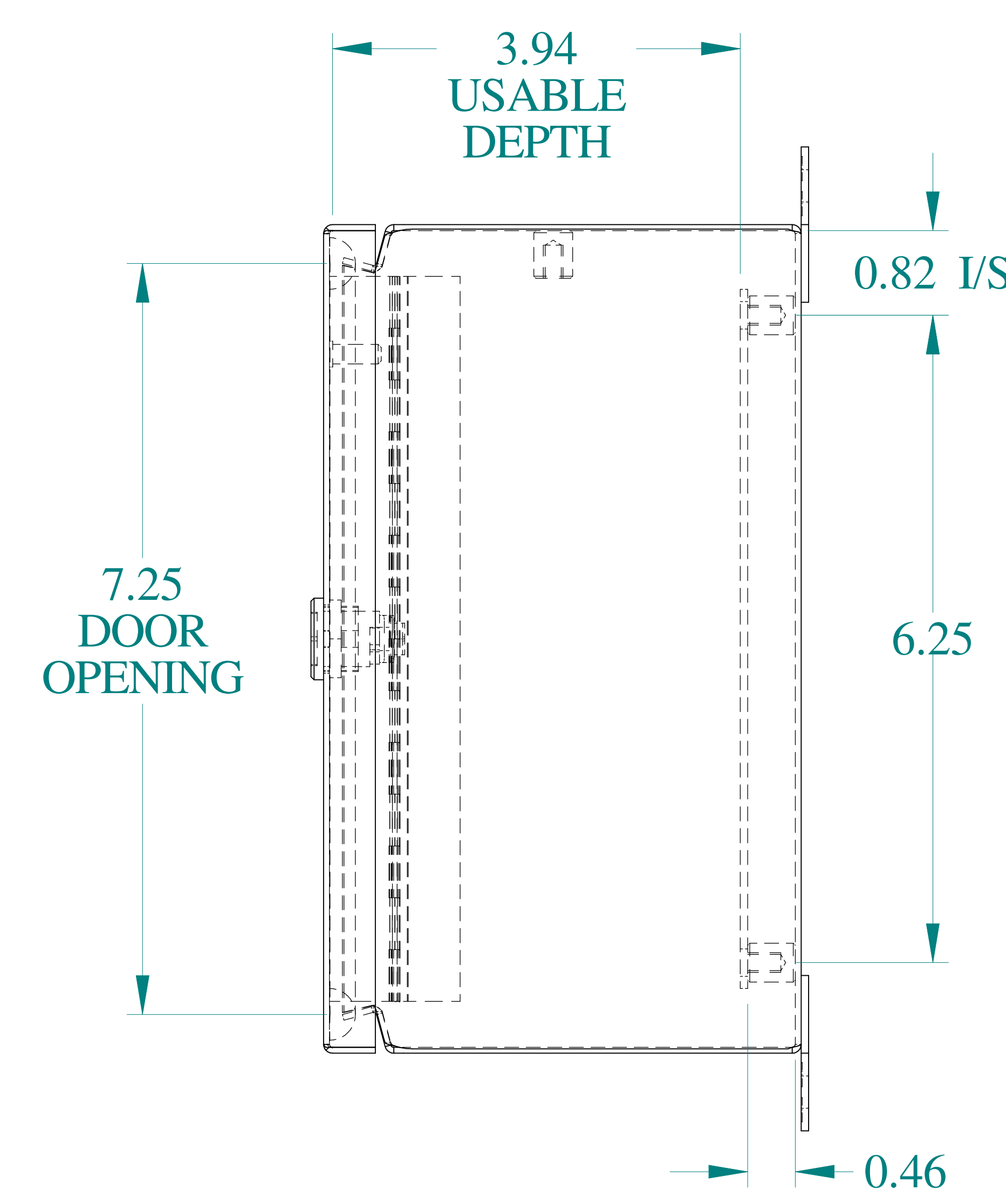
SIDE VIEW
