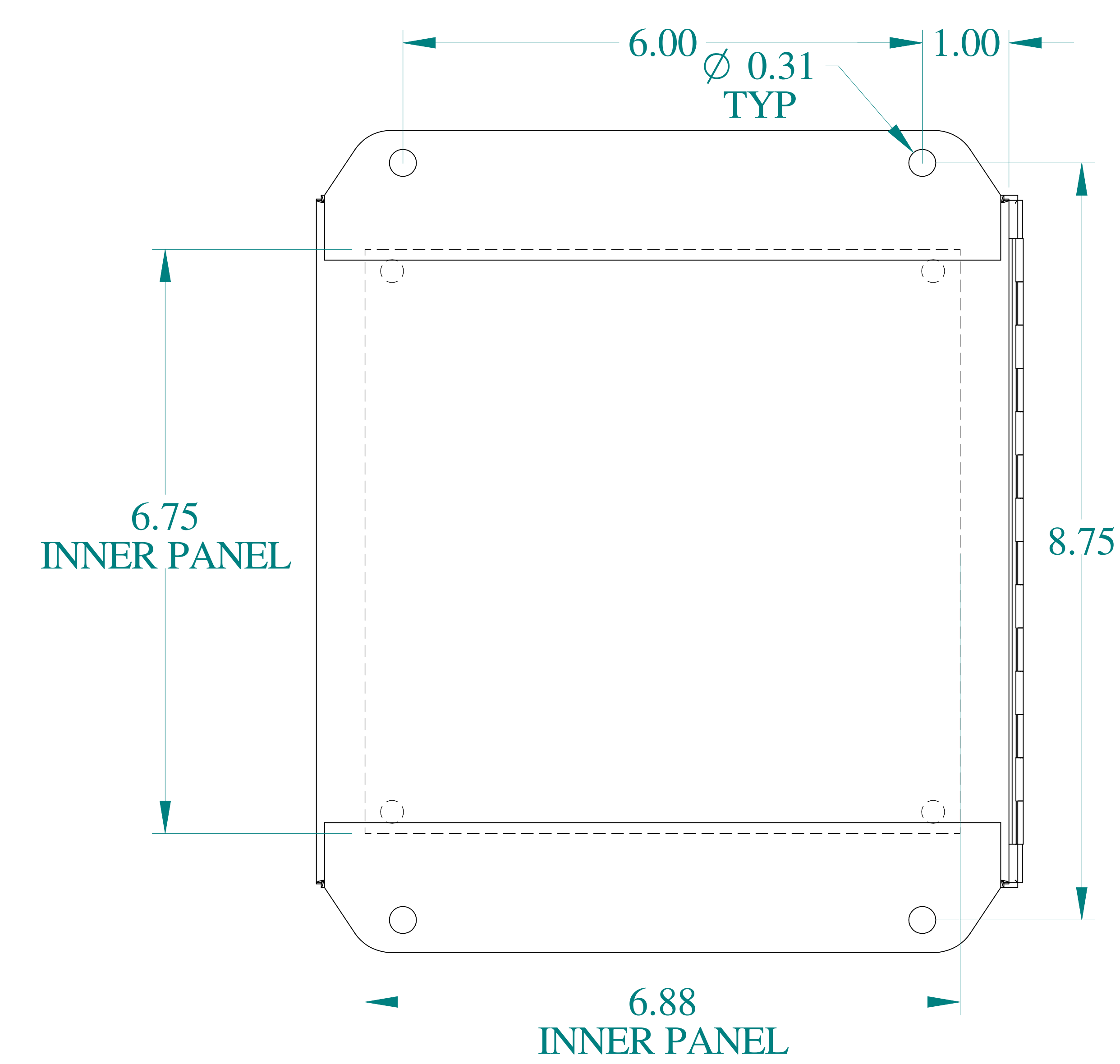
BACK VIEW
